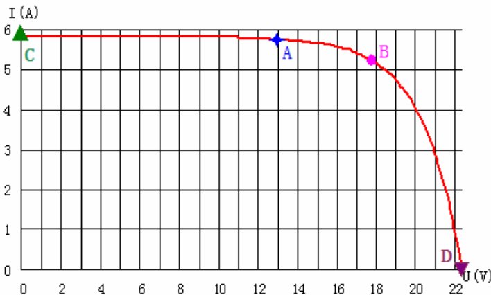
Figure 2-4: Voltage-Current Curve
