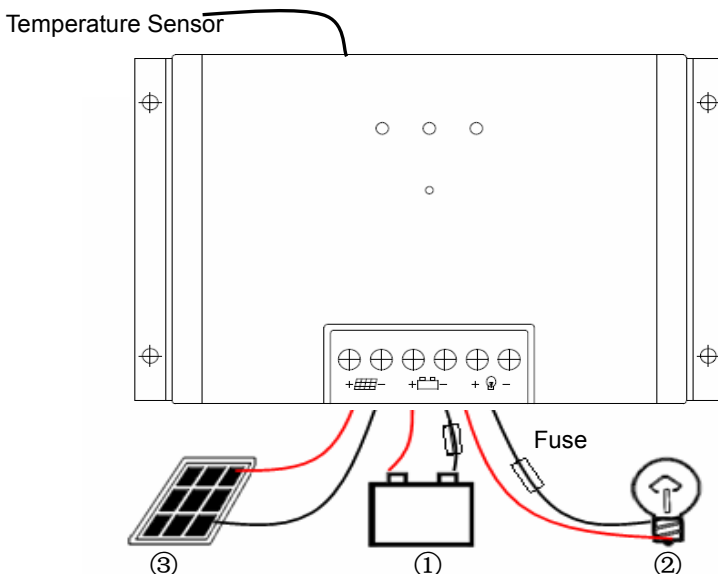
Figure 4-2: Connecting Diagram
