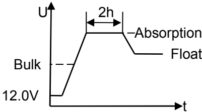
Figure 2-2: Three-stage Charge
