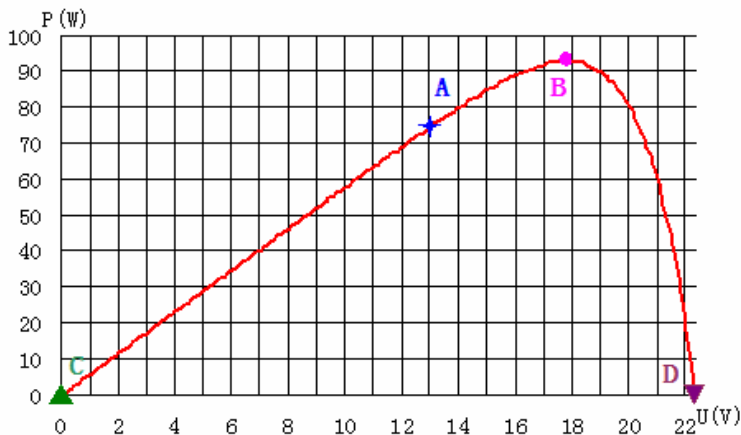
Figure 2-5: Voltage-Power Curve
