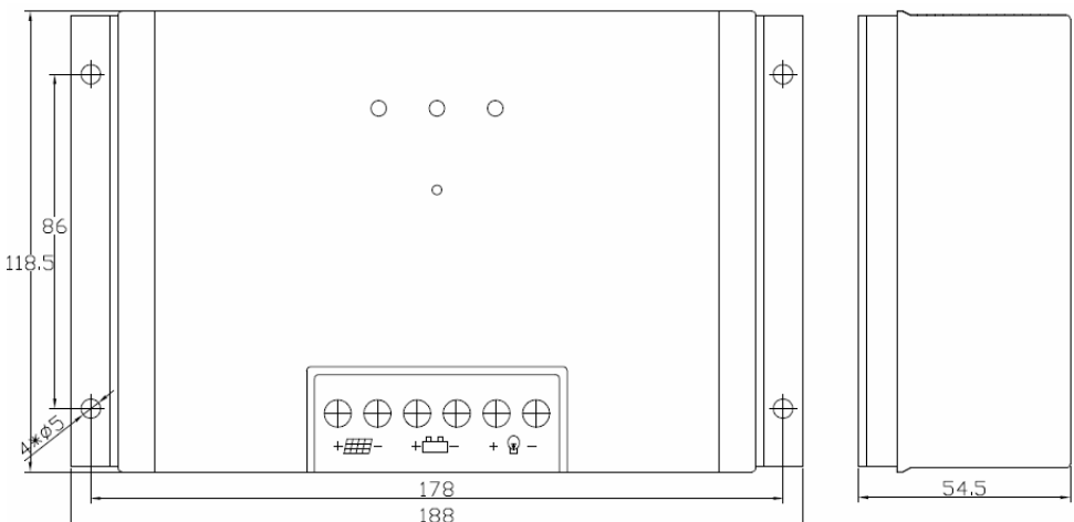
Figure 4-1: Dimensions (Unit: mm)
